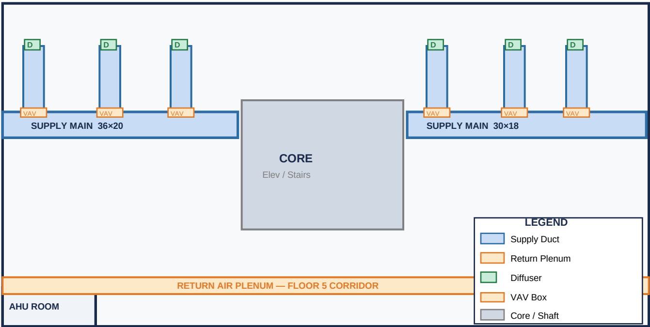
Figure 2 — Typical Floor Duct Layout, Floor 5 (Schematic — Not to Scale)
